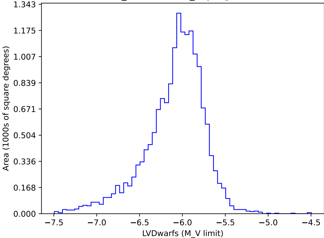
weather_cloudso8v3.5_10yrs gi: LVDwarfs
