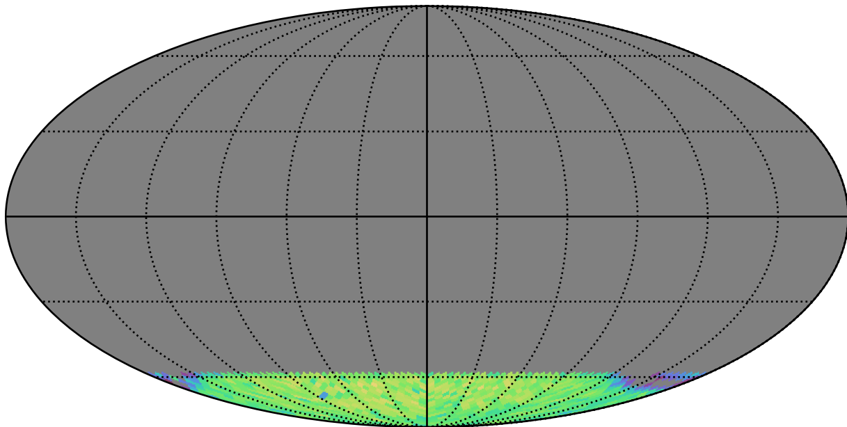
weather_cloudso8v3.5_10yrs gi SCP: LVDwarfs
