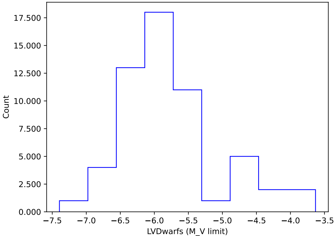
weather_cloudso8v3.5_10yrs gi: LVDwarfs
