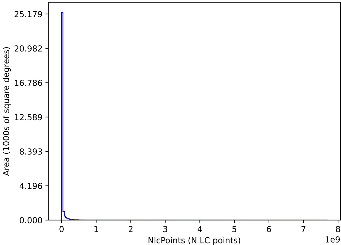
weather_cloudso8v3.5_10yrs : NlcPoints
