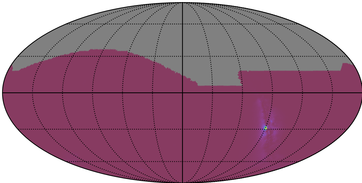
weather_cloudso8v3.5_10yrs : NlcPoints
