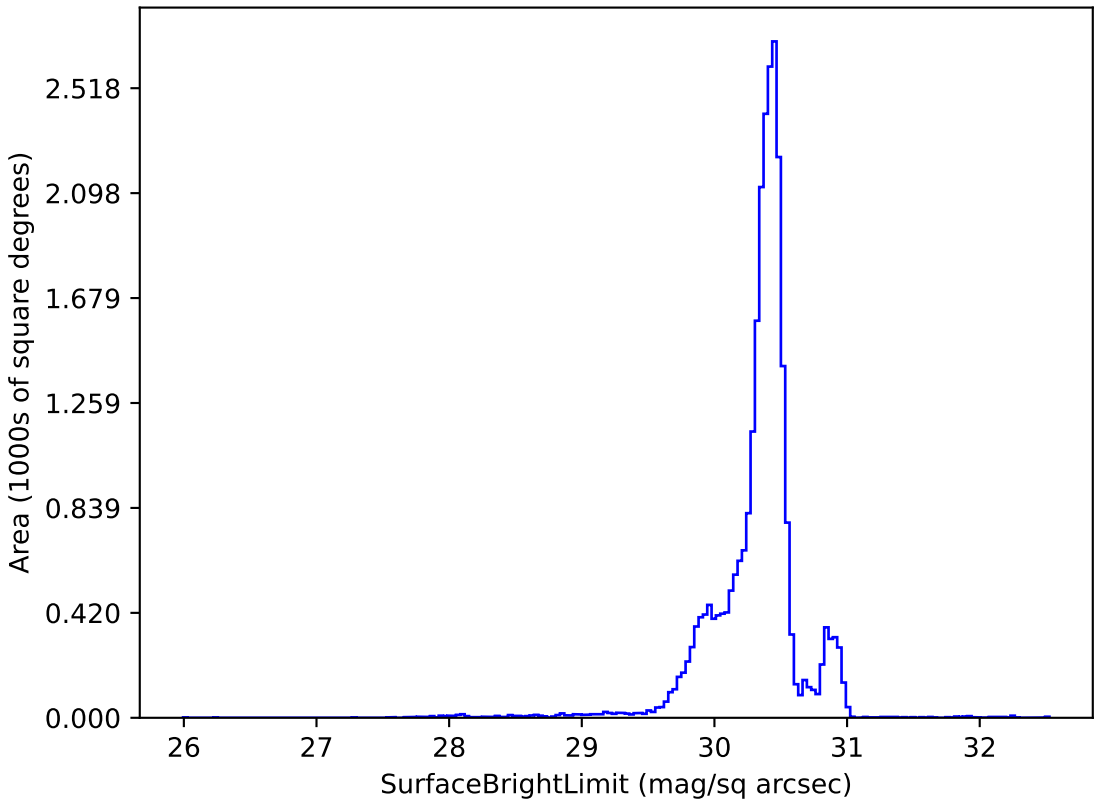
weather_cloudso8v3.5_10yrs g: SurfaceBrightLimit
