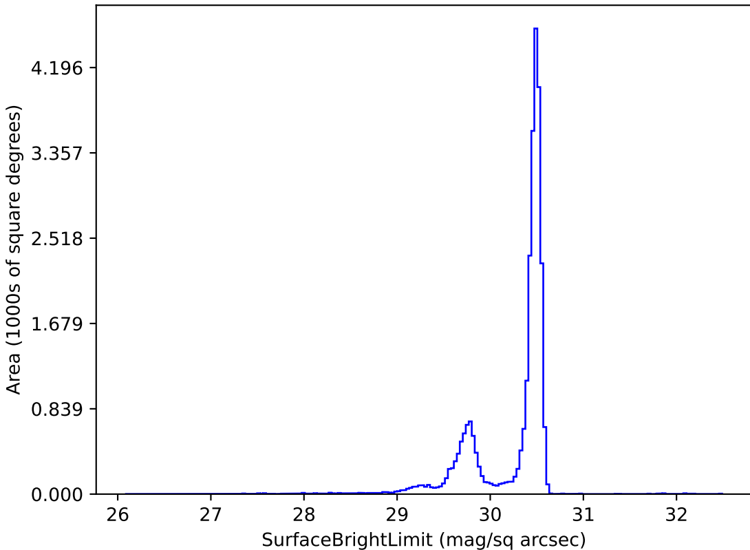
weather_cloudso8v3.5_10yrs r: SurfaceBrightLimit
