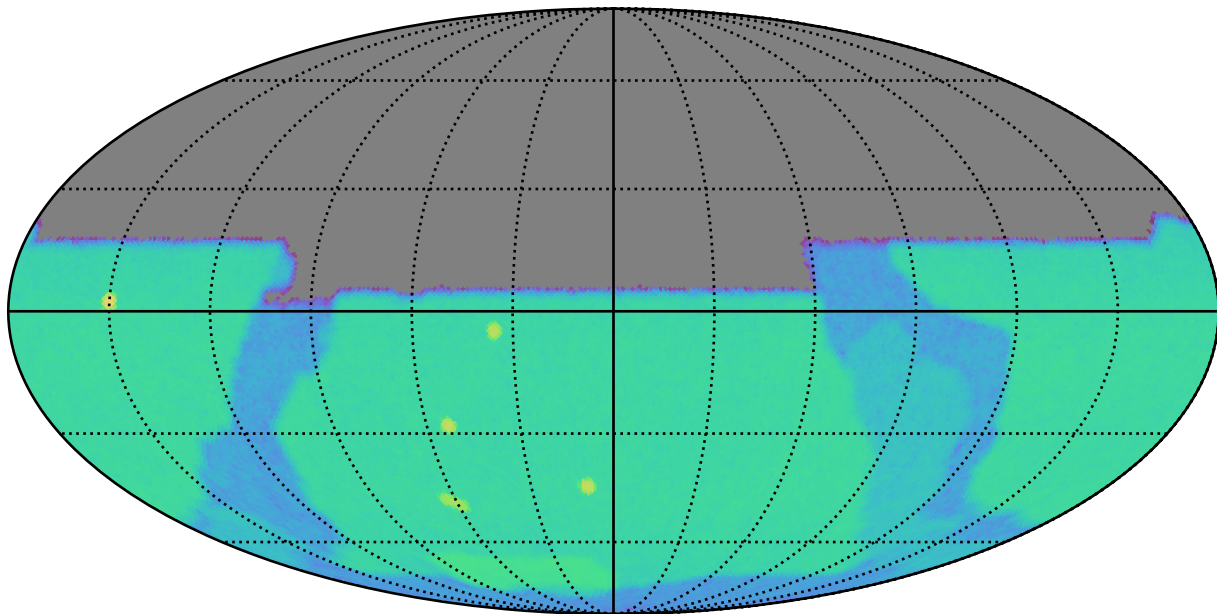
weather_cloudso8v3.5_10yrs u: SurfaceBrightLimit
