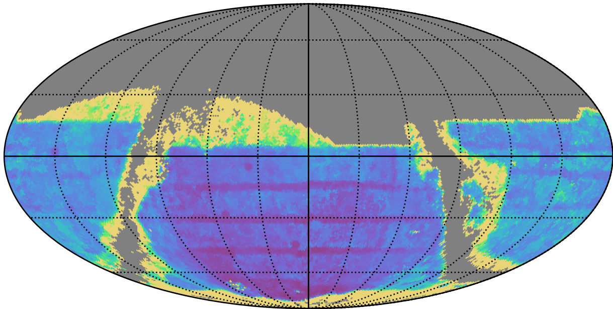
weather_cloudso8v3.5_10yrs : TDC_accuracy
