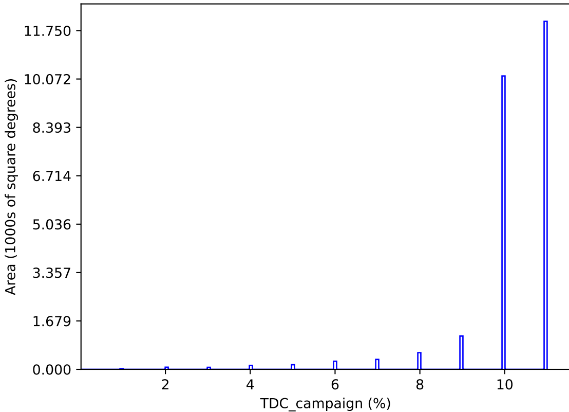
weather_cloudso8v3.5_10yrs : TDC_campaign
