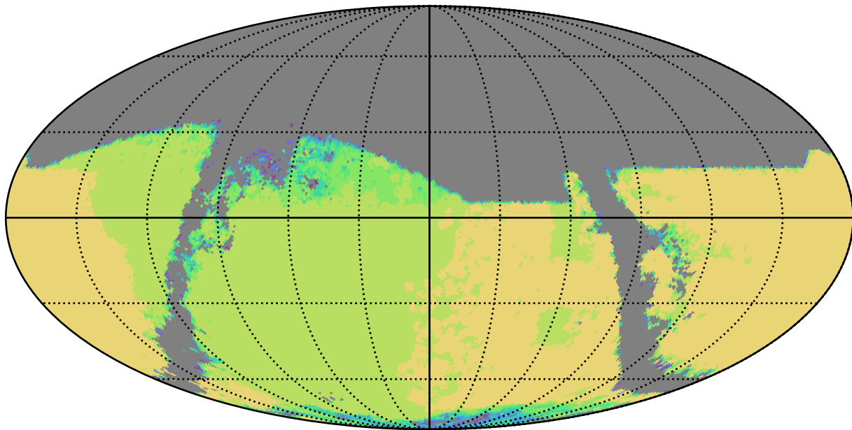
weather_cloudso8v3.5_10yrs : TDC_campaign
