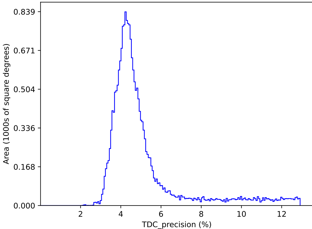
weather_cloudso8v3.5_10yrs : TDC_precision
