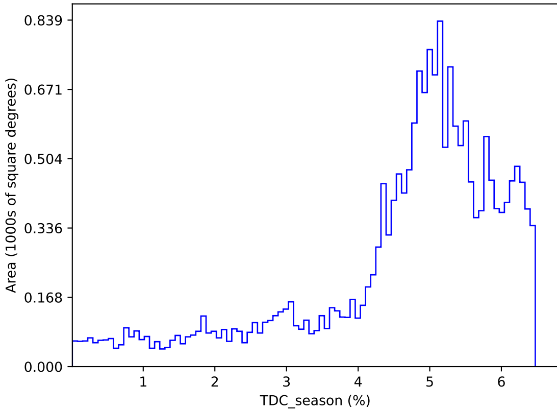
weather_cloudso8v3.5_10yrs : TDC_season
