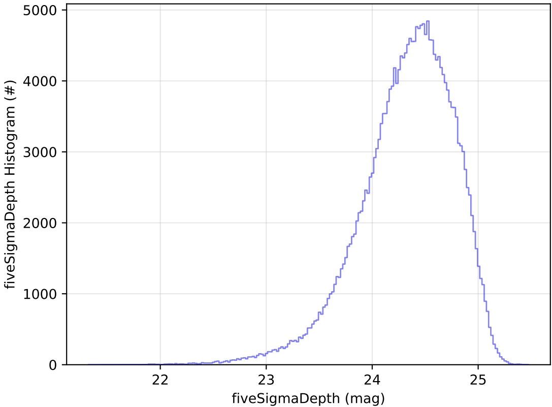
weather_cloudso8v3.5_10yrs g: fiveSigmaDepth Histogram
