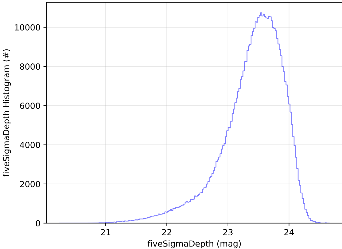
weather_cloudso8v3.5_10yrs i: fiveSigmaDepth Histogram
