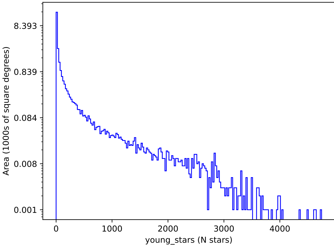
weather_cloudso8v3.5_10yrs : young_stars
