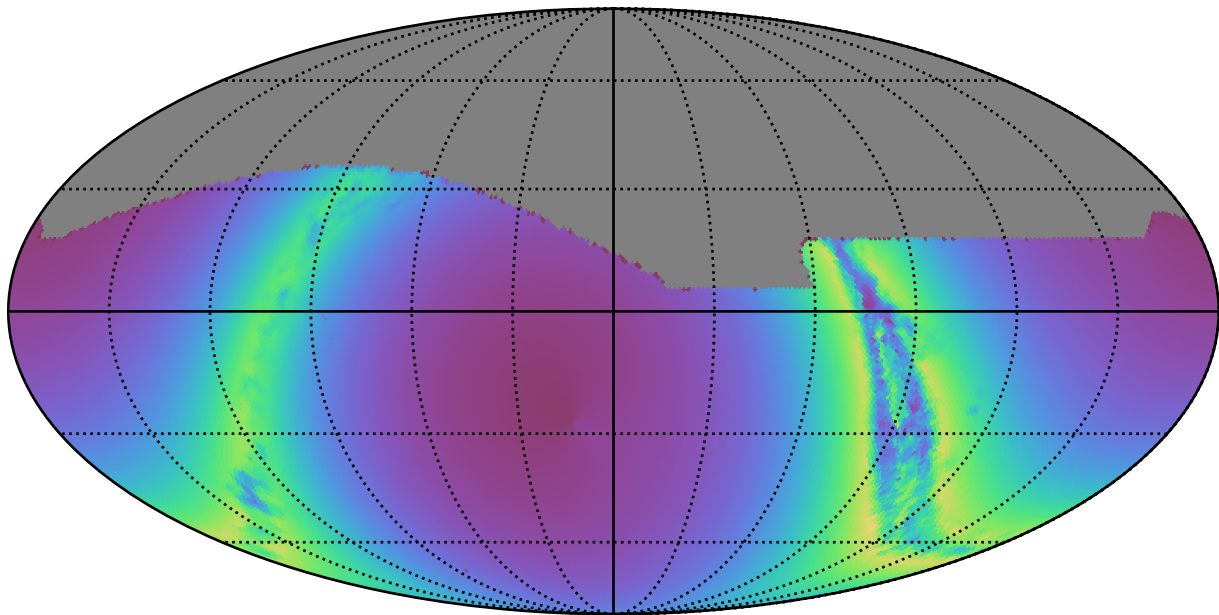
weather_cloudso8v3.5_10yrs : young_stars
