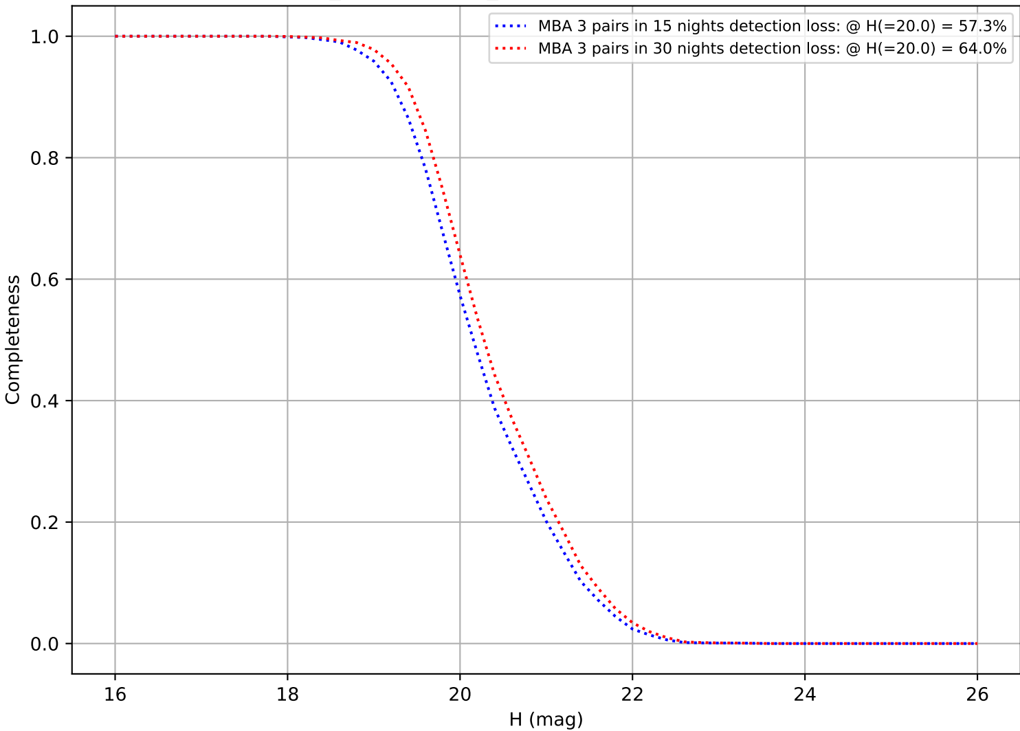
weather_cloudso8v3.5_10yrs: DifferentialCompleteness
