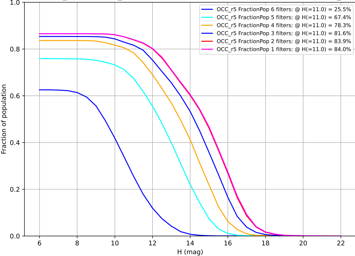
weather_cloudso8v3.5_10yrs: Fraction of population with colors in X filters OCC_r5
