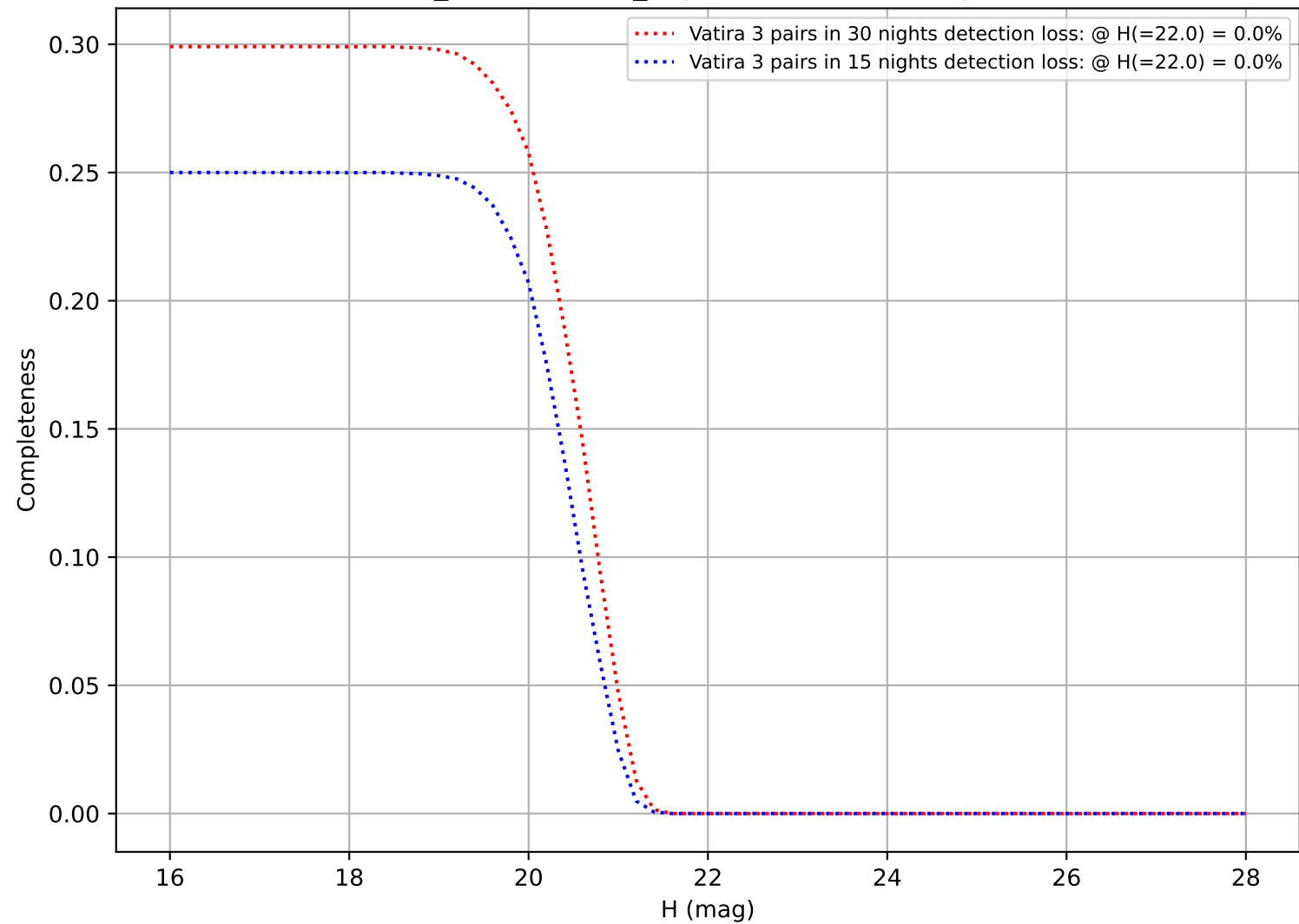
weather_cloudso8v3.5_10yrs: DifferentialCompleteness
