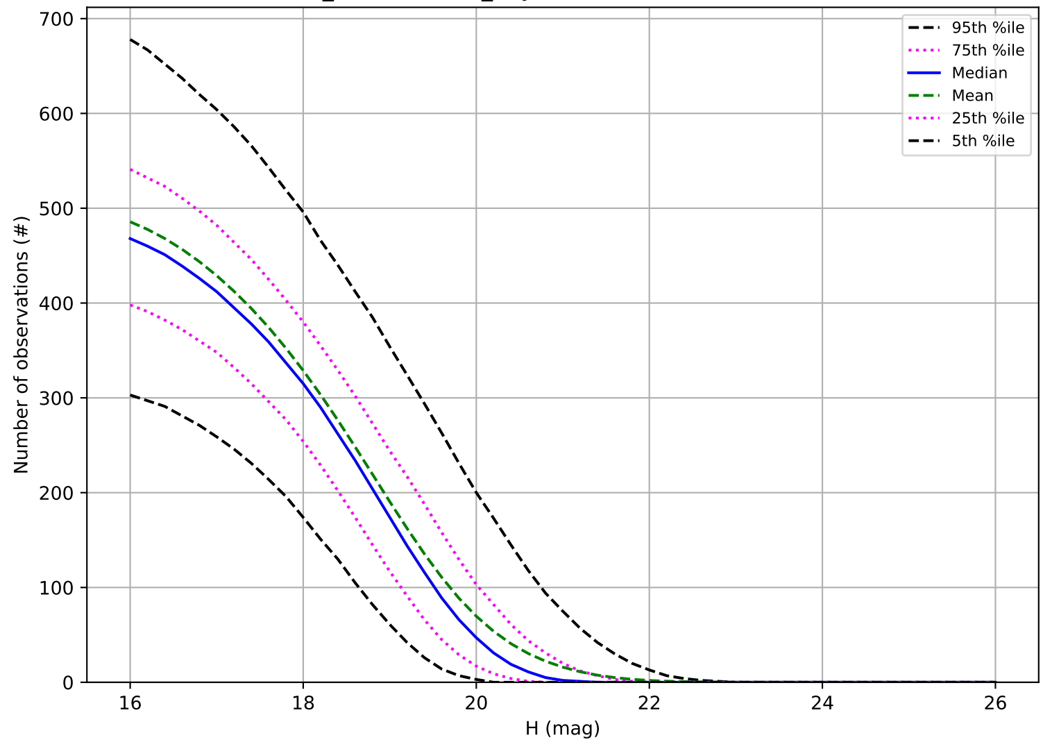
weather_cloudso8v3.5_10yrs: Number of observations MBA
