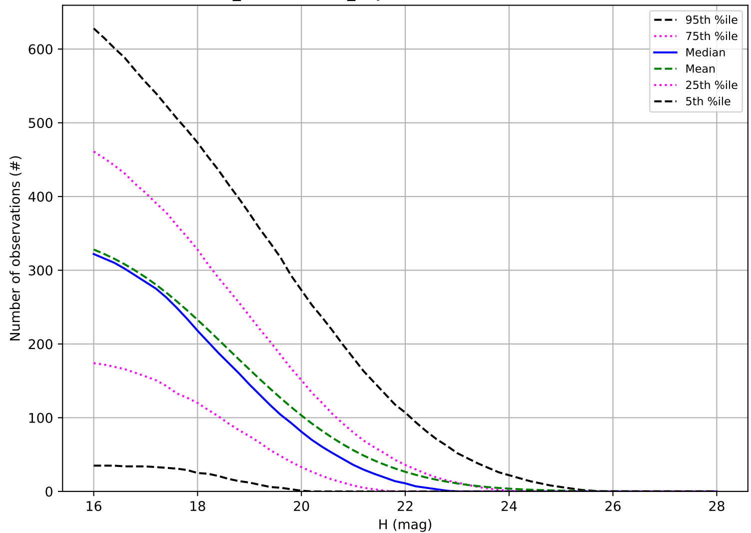
weather_cloudso8v3.5_10yrs: Number of observations NEO
