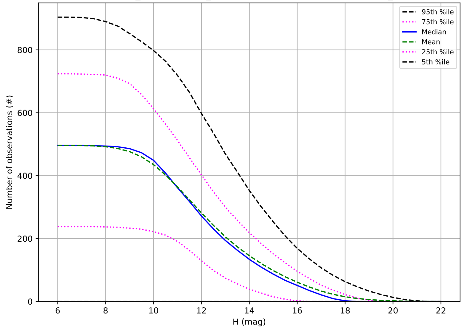
weather_cloudso8v3.5_10yrs: Number of observations OCC_r5
