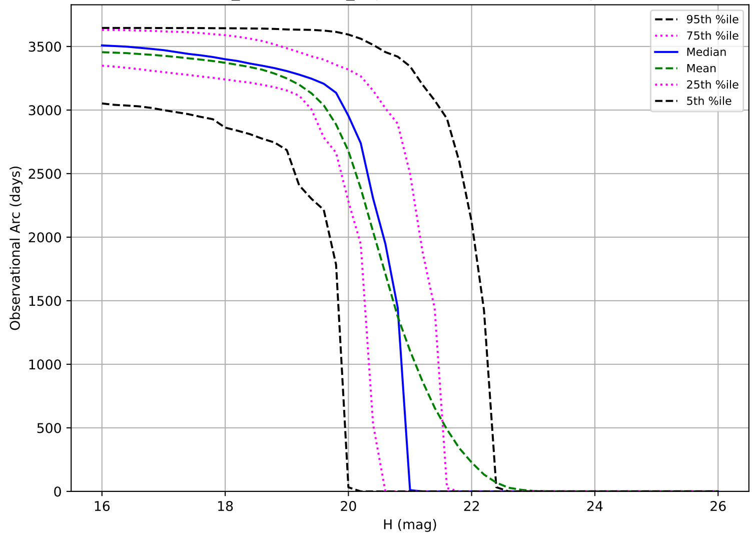
weather_cloudso8v3.5_10yrs: Observational Arc Length MBA
