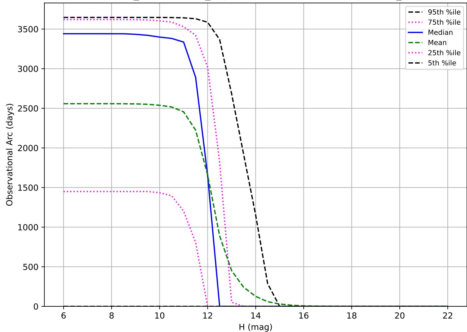
weather_cloudso8v3.5_10yrs: Observational Arc Length OCC_r20
