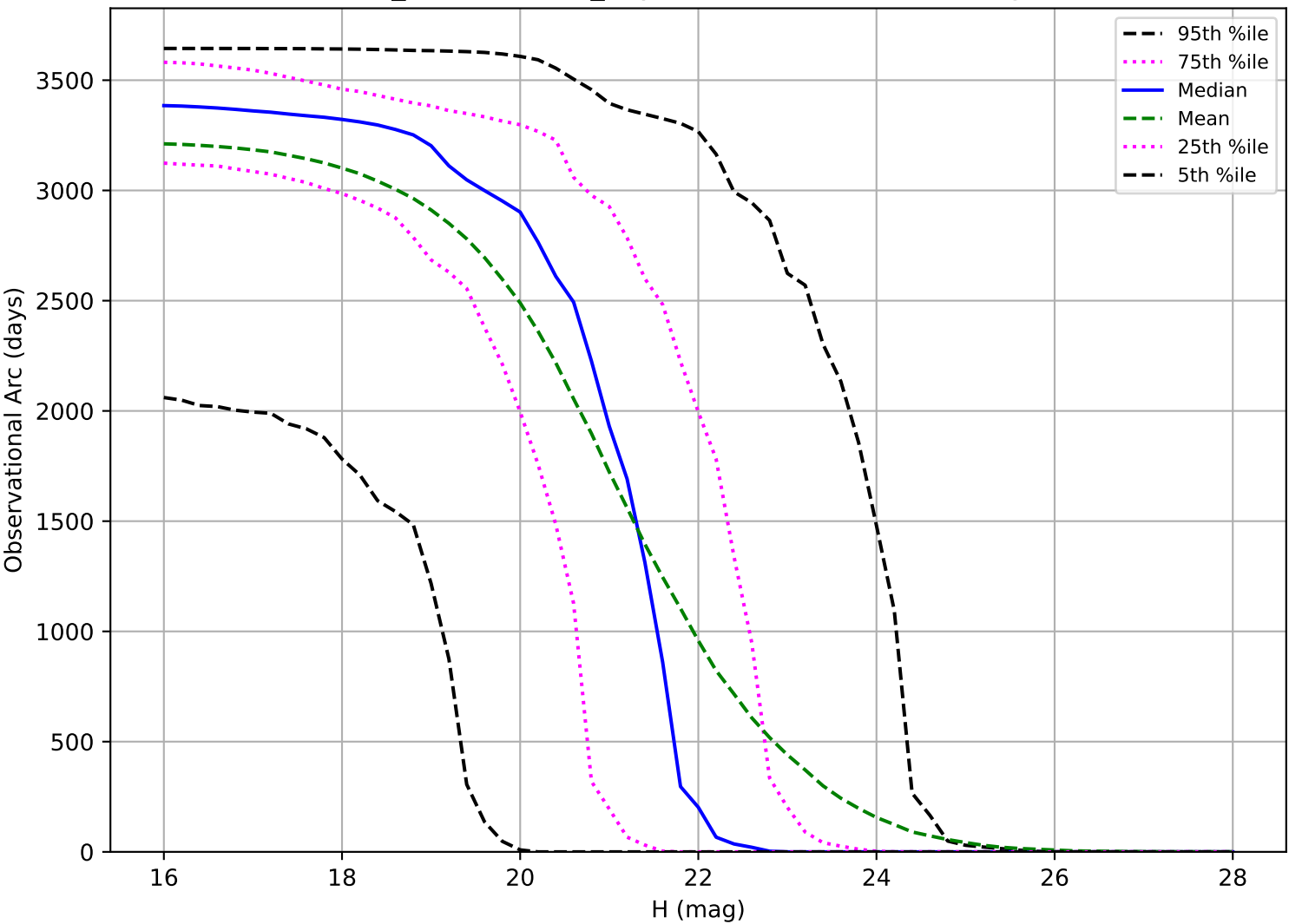
weather_cloudso8v3.5_10yrs: Observational Arc Length PHA
