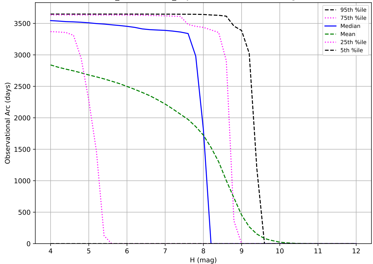
weather_cloudso8v3.5_10yrs: Observational Arc Length TNO
