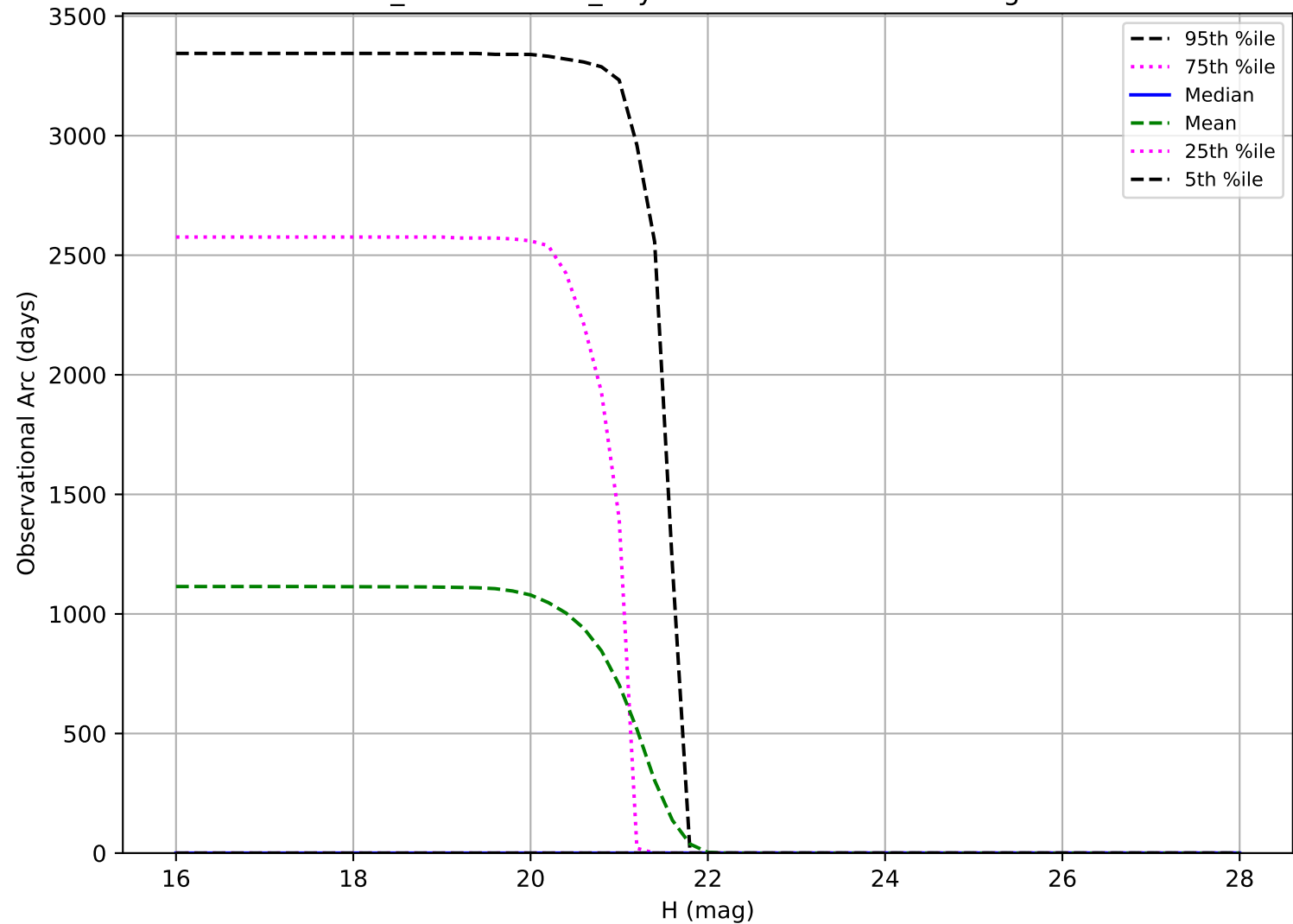
weather_cloudso8v3.5_10yrs: Observational Arc Length Vatira
